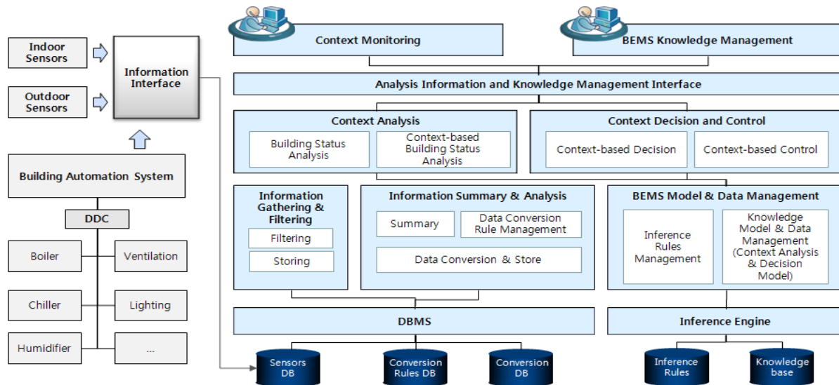
Fig. 1: System architecture of the proposed BEMS model
