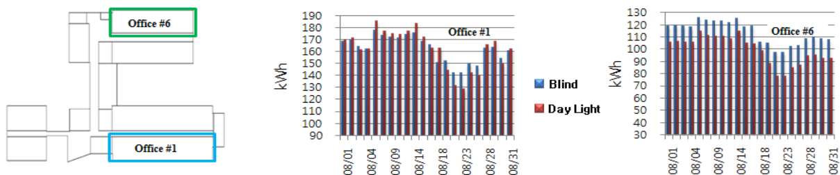
Fig. 5: Comparison of energy consumption in the day lighting simulation
