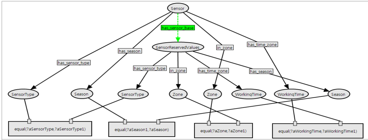
Fig. 2: Instance of inference rules generation
