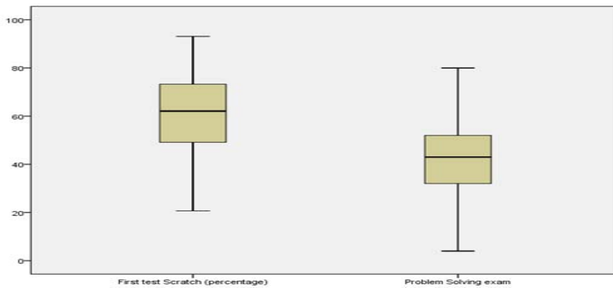
Fig. 3: Box-and-Whisker Plot
