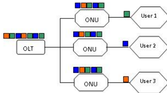
Fig. 2: Upstream transmission
