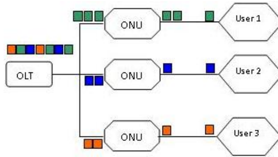
Fig. 1: downstream transmission
