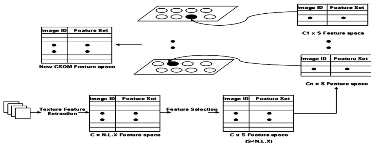
Fig. 3: Generated Features based CSOM.
