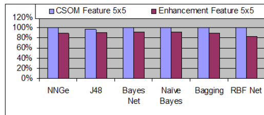
Fig.4: The Classification Rate Comparison.
