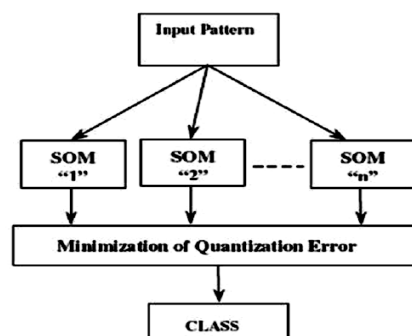
Fig.2: The CSOM Model (classification phase).
