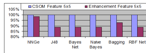
Fig. 5: The Classification Rate Comparison.
